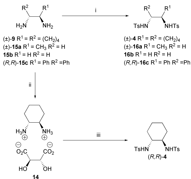
Scheme 3 Reagents and conditions: i, TsCl, \text{Et}_3\text{N} or ^i\text{PrNEt}_2 , \text{CH}_2\text{Cl}_2 , 68–79%; ii, (a) L-(+)-(2 R ,3 R ) tartaric acid, 70 °C, (b) AcOH, 90 °C, 85%; iii, TsCl, 1.2 N NaOH, \text{CH}_2\text{Cl}_2 , 85%.
