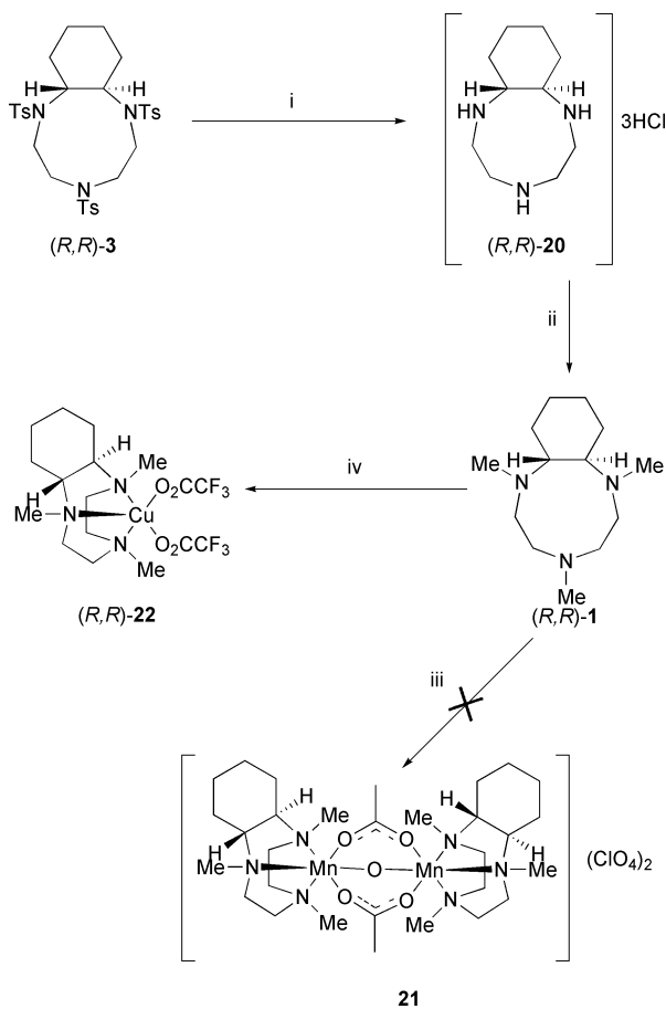
Scheme 5 Reagents and conditions: i, (a) Li, NH 3 , EtOH, (b) aq. HCl (73%); ii, (a) aq. NaOH, (b) HCO 2 H, HCHO, Δ, 24 h (79%); iii, Mn(OAc) 2 , MeOH–H 2 O (9 : 1), NaClO 4 ; iv, (a) CuCl 2 , CH 3 CN (b) Ag 2 O 2 CCF 3 .
