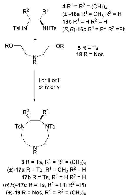
Scheme 4 Reagents and conditions: i, (method A) \text{K}_2\text{CO}_3 , DMF, 50 °C, 7 d; ii, (method B) (a) NaOEt, EtOH (b) 5 , DMF, 100 °C; iii, (method C) (a) 2 equiv. NaH, DMF, (b) 5 , DMF, 70 °C; iv (method D) disodium salt of 16a , 5 , DMSO, 100 °C; v, (method E) (a) 2 equiv. LiH, DMF, 70 °C, (b) 5 or 18 , DMF, 50 °C, 7 d.
