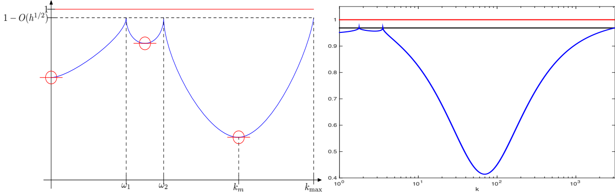
FIGURE 3. Left: drawing of the optimized convergence factor \rho_{opt} studied in Theorem 3 for the case \alpha = \beta . Right: actual plot of the optimized convergence factor from Theorem 3 for \mu_1 = \mu_2 = 1 , \varepsilon_1 = 1 , \varepsilon_2 = 4 , \omega = \pi and h = 10^{-3} . The red line is at 1 and the black line is the asymptotic maximum ( 1 - \mathcal{O}(h^{\frac{1}{2}}) for this case).
