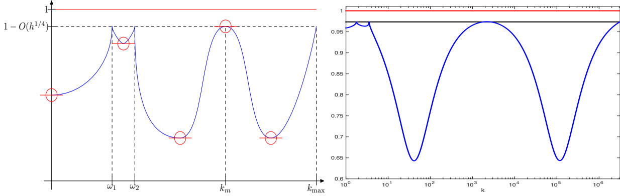
FIGURE 1. Left: drawing of the optimized convergence factor \rho_{opt} studied in Theorem 3. Right: actual plot of the optimized convergence factor from 3 for \mu_1 = \mu_2 = 1 , \varepsilon_1 = 1 , \varepsilon_2 = 4 , \omega = \pi and h = 10^{-6} . The red line is at 1 and the black line is the asymptotic maximum ( 1 - \mathcal{O}(h^{\frac{1}{4}}) for this case).
