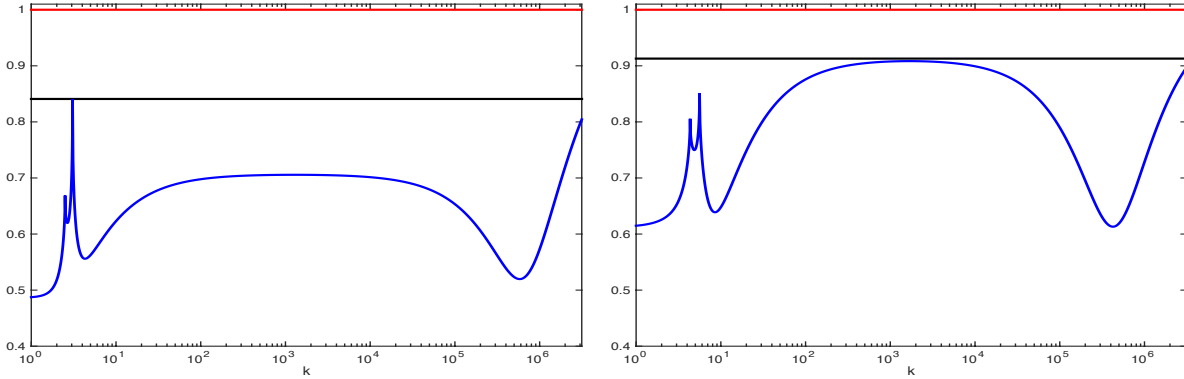
FIGURE 5. Convergence factor \rho_{opt} from the third and fourth case of Theorem 5 ( \varepsilon_2 < \varepsilon_1 ). The red line is 1, the black line is the asymptotic maximum: \sqrt[4]{\frac{1}{2}} for the left case with \mu_1 = \varepsilon_2 = \mu_2 = 1 , \varepsilon_1 = 2 , \omega = \pi and h = 10^{-6} and \varepsilon for the right case with \varepsilon_1 = 6 , \varepsilon_2 = 5 , \mu_1 = 1 , \mu_2 = 1 , \omega = \pi and h = 10^{-6} . Convergence does not depend on the mesh size h .
