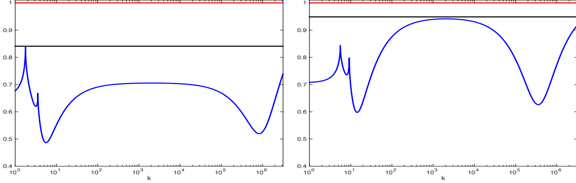
FIGURE 4. Convergence factor \rho_{opt} from the first and the second case of Theorem 5 ( \varepsilon_1 < \varepsilon_2 ). The red line denotes 1, the black line is the asymptotic maximum: \sqrt[4]{\frac{1}{2}} for the left case with \mu_1 = \varepsilon_1 = \mu_2 = 1 , \varepsilon_2 = 2 , \omega = \pi and h = 10^{-6} , and \varepsilon for the right case with \varepsilon_1 = 9 , \varepsilon_2 = \mu_1 = \mu_2 = 10 , \omega = \pi and h = 10^{-6} . Convergence does not depend on the mesh size h .
