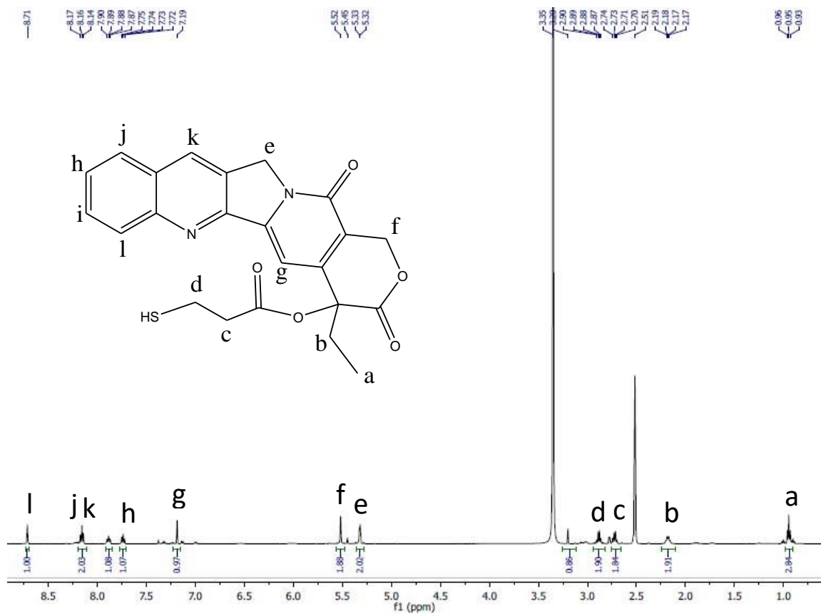
Figure S1. ^1\text{H} -NMR spectrum of thiolated camptothecin CPT-SH (in DMSO- d_6 , 500 MHz).
