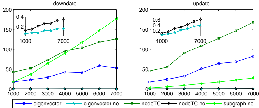
FIG. 6. Timings in seconds for scale-free graphs of increasing size (500 modifications).
